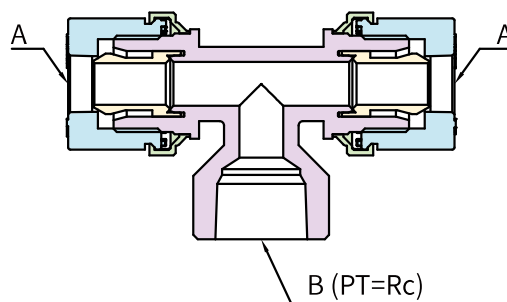
FEMALE TEE
