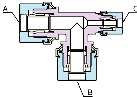
REDUCING UNION TEE
