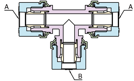
REDUCING UNION TEE
