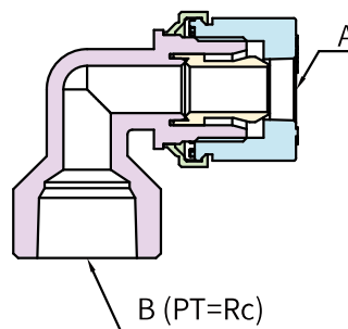
FEMALE ELBOW
