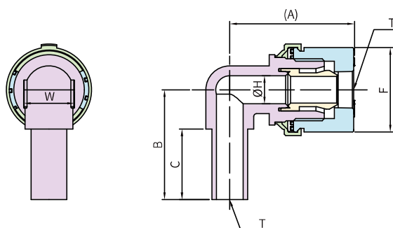
▲ TUBE END TYPE
