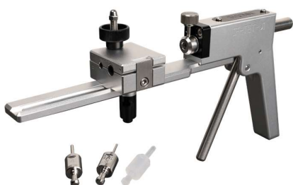
Tube Expanding Gun
