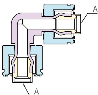
ELBOW ADAPTOR (SLEEVE & NUT SET)
