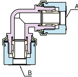
REDUCING UNION ELBOW
