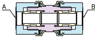
REDUCING UNION CONNECTOR
