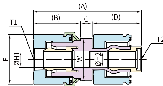
▲ SLEEVE & NUT SET
