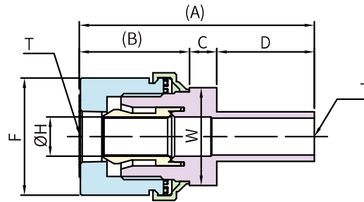
▲ TUBE END TYPE
