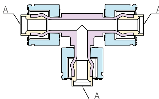
TEE ADAPTOR (SLEEVE & NUT SET)
